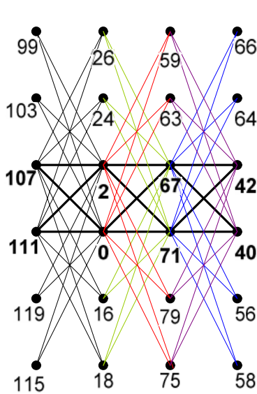
Figure (11a) m \equiv 0 \pmod{2} ,
