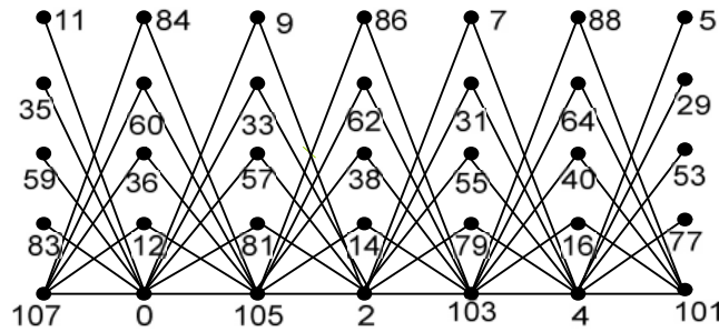
Figure 8: The graph Spl_4(P_7) with its odd graceful labeling.
