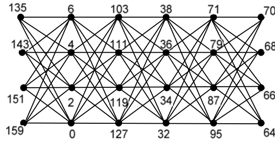
Figure 1: The graph D_4(P_6) with its odd graceful labeling.
