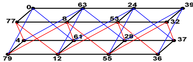
Figure 6: The graph D_2(P_n \times P_2) with its odd graceful labeling.
