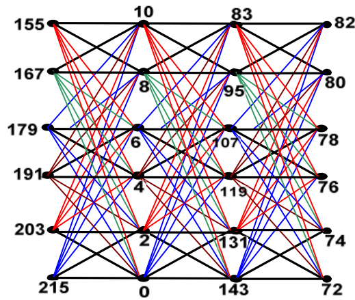
Figure 4: The graph D_3(P_4 \oplus \overline{K_2}) with its odd graceful labeling.
