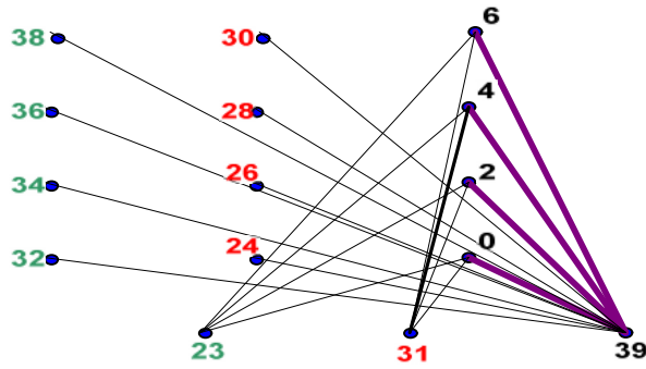
Figure 9: The graph spl_2(K_{1,4}) with its odd graceful labeling.
