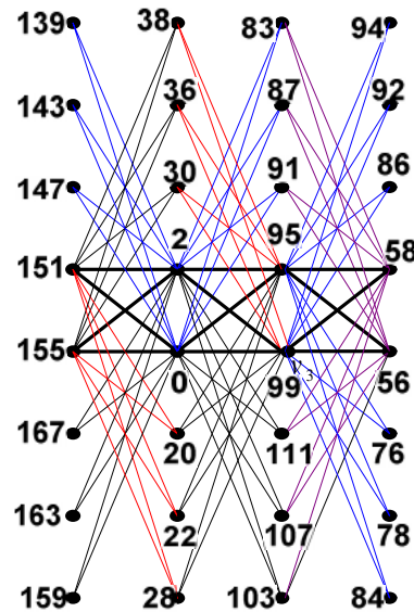
Figure (11b), m \equiv 1 \pmod{2}
